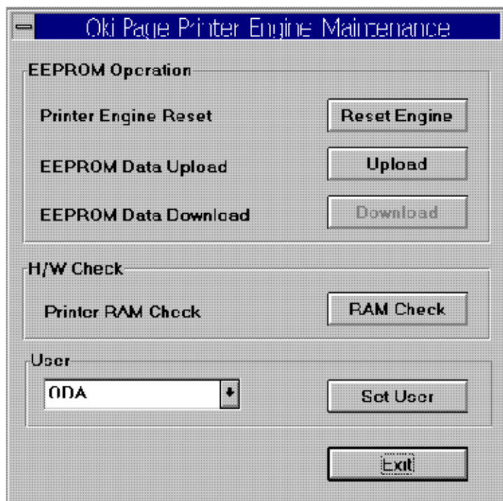
Figure C-2 Option Menu Dialog (Preliminary)
