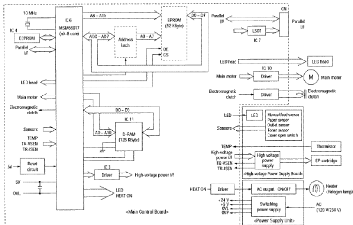
Figure 2-1 Block Diagram
