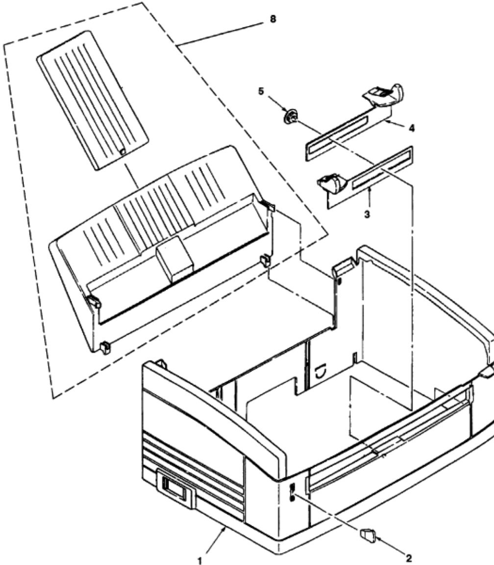
Figure 8-1 Cover Assy Upper
