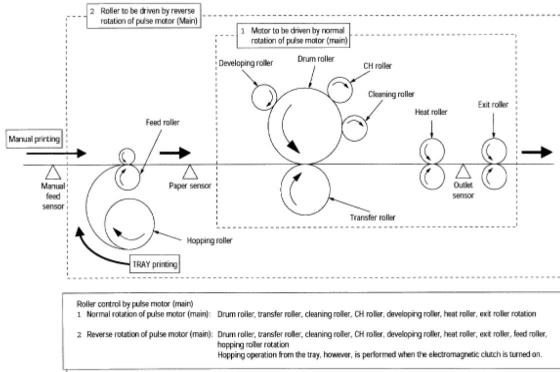
Figure 2-4 Schematic Drawing of OKIPAGE 4w Paper Feeding
