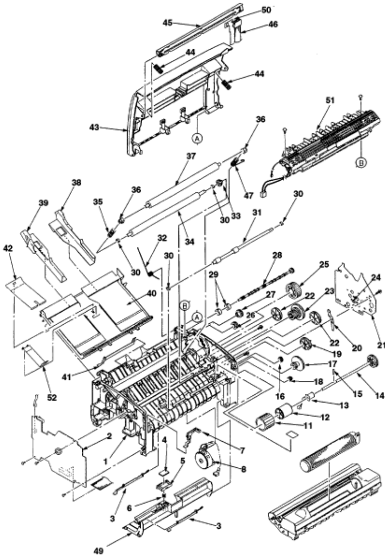
Figure 8-2 Base Frame Unit
