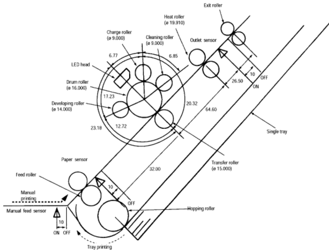
Figure 2-3 Layout Drawing of Electro-Photographic Processor
